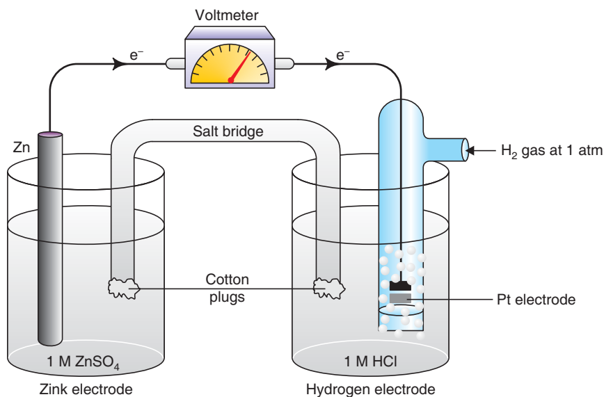
Figure 4.8 Standard Hydrogen Electrode
